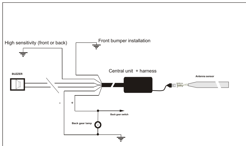
Block schematic
